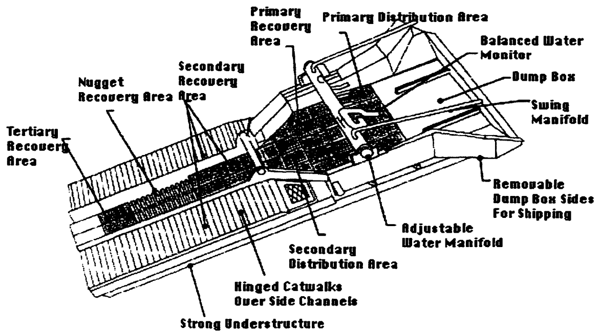
Figure 3.3: A Gold Sluice Diagram
